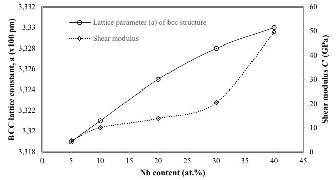
Figure 1: Effect of niobium content on lattice parameter and shear modulus Ti-Nb x -Ta 25 -Zr 5 alloys at 0 K
